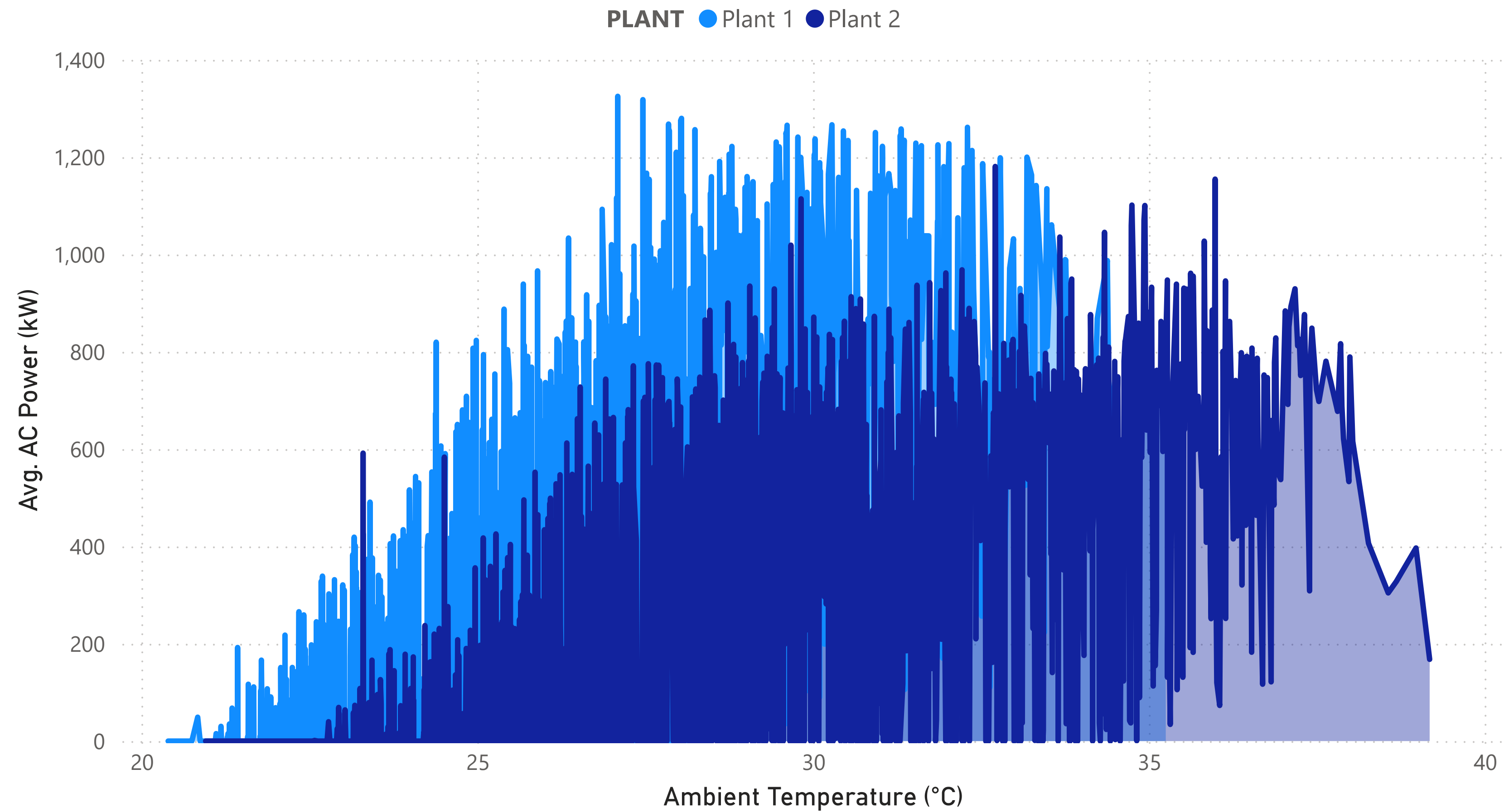
Ambient Temp. vs Avg. AC Power
