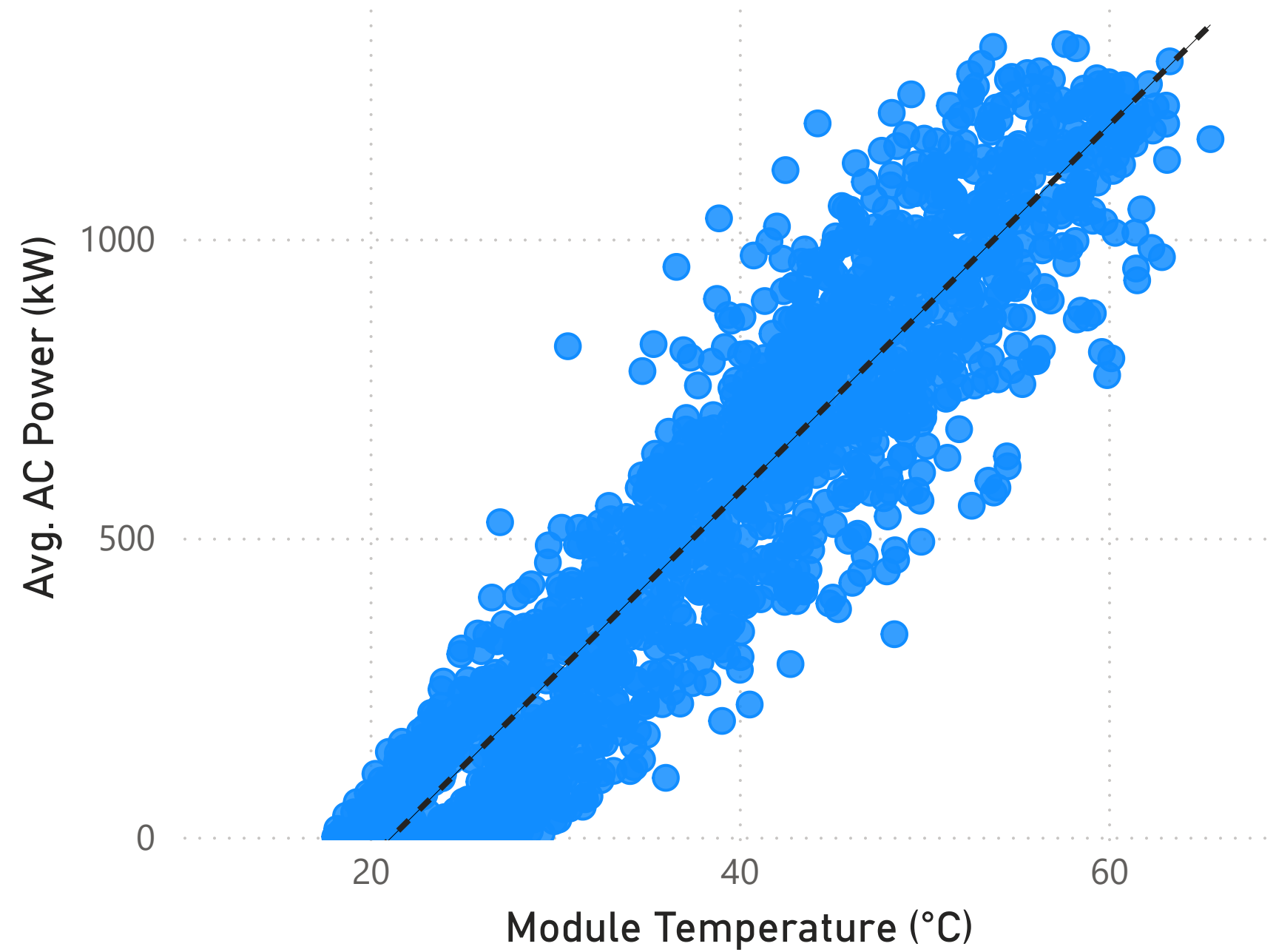
Module Temperature vs AC Power - Plant 2
